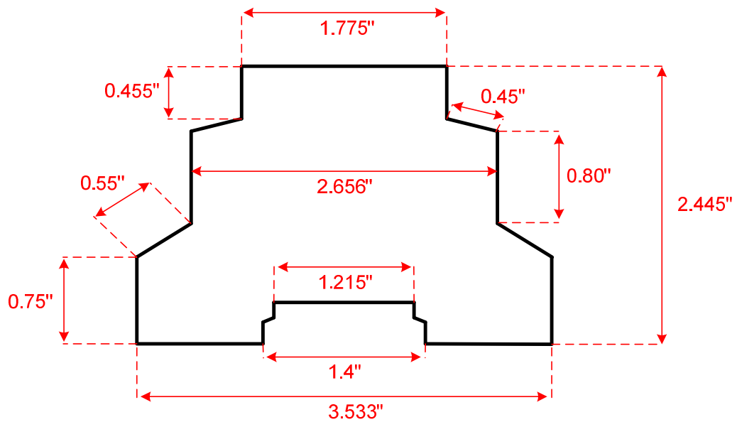
Side View
